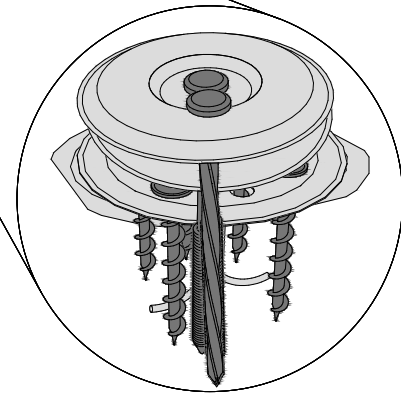
SOPREMA FASTENERS FOR CONCRETE WITH CORRUGATED CONCRETE
