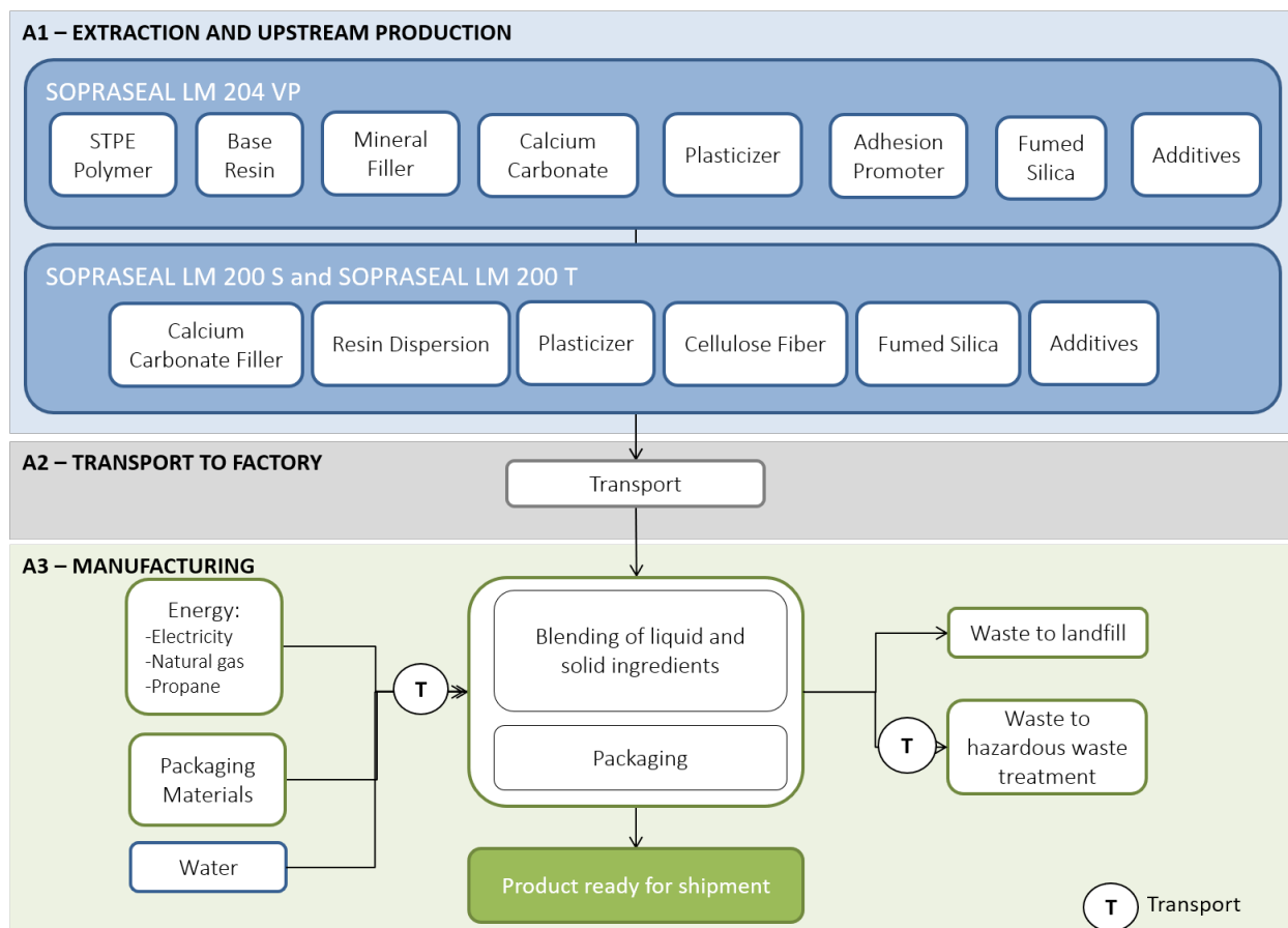
Figure 1: System Boundaries of Cradle-to-Gate LCA of SOPREMA's SOPRASEAL LM 200 S, LM 200 T and LM 204 VP liquid applied membranes.
