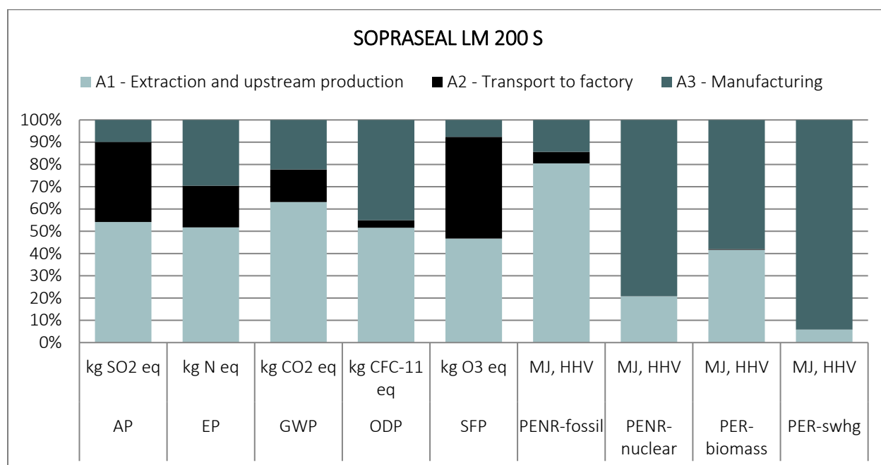
Contribution analysis of information modules A1-A3 of the SOPRASEAL LM 200 S product life cycle stage - TRACI & CED indicators.
