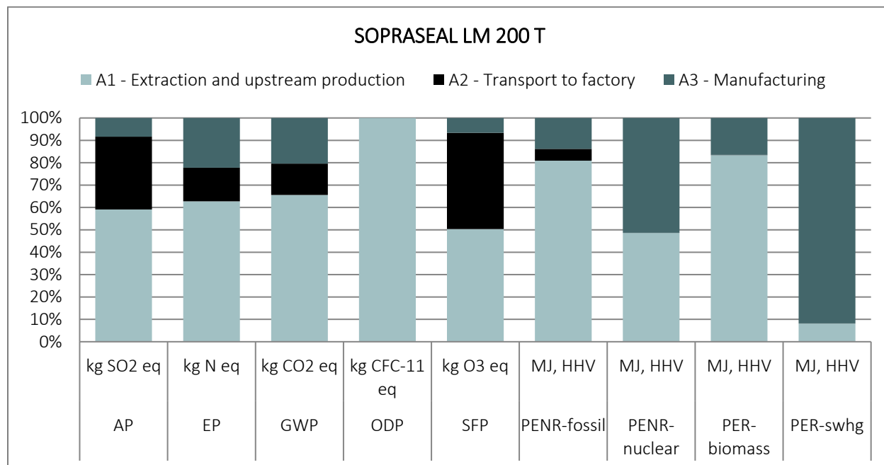
Contribution analysis of information modules A1-A3 of the SOPRASEAL LM 200 T product life cycle stage - TRACI & CED indicators.
