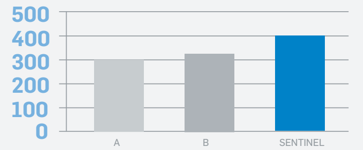
BREAKING STRENGTH - 200 lbf/in, minimum per ASTM D4434
